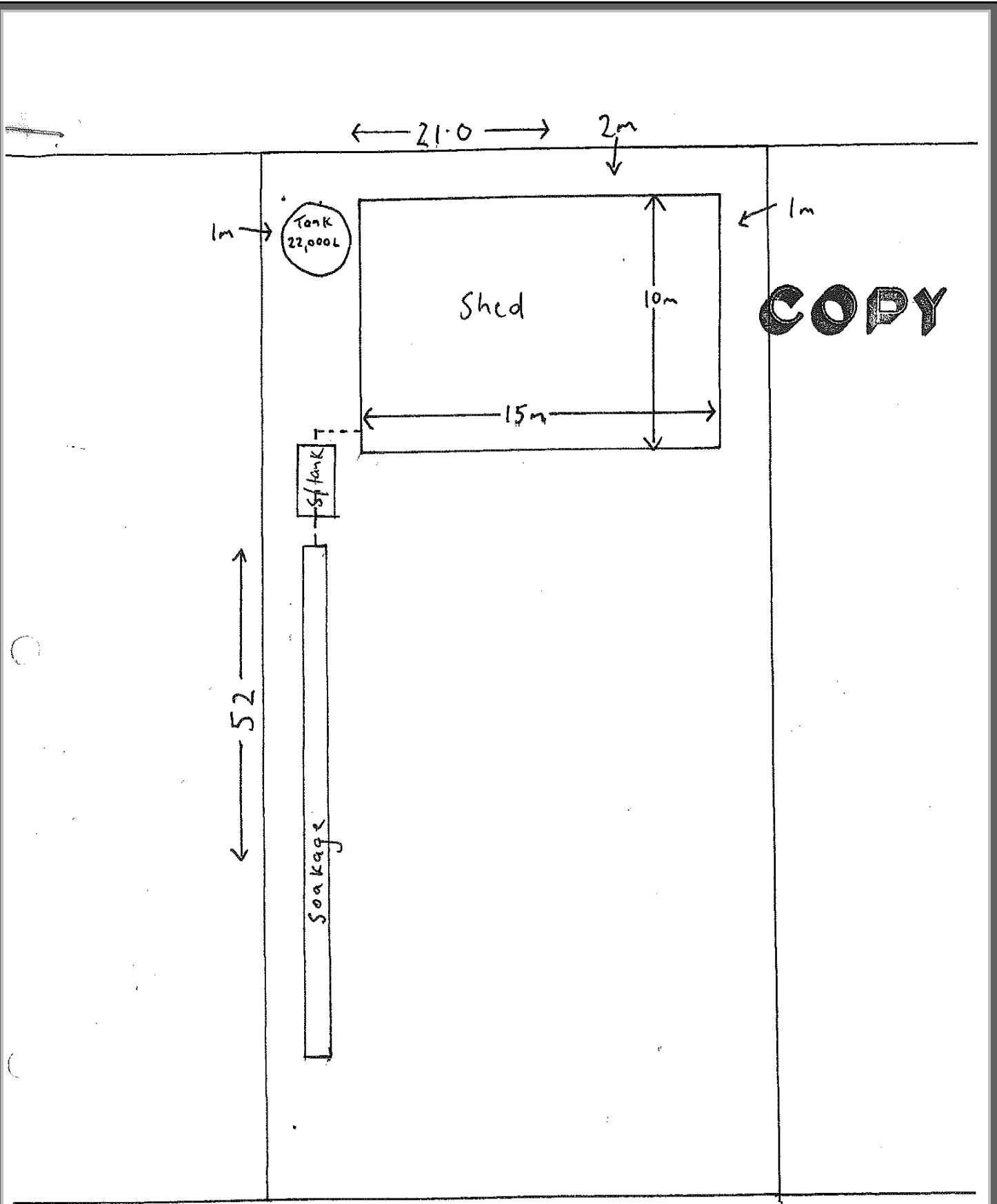
EXAMPLE OF SITE PLAN FOR SEPTIC TANK INSTALLATION
